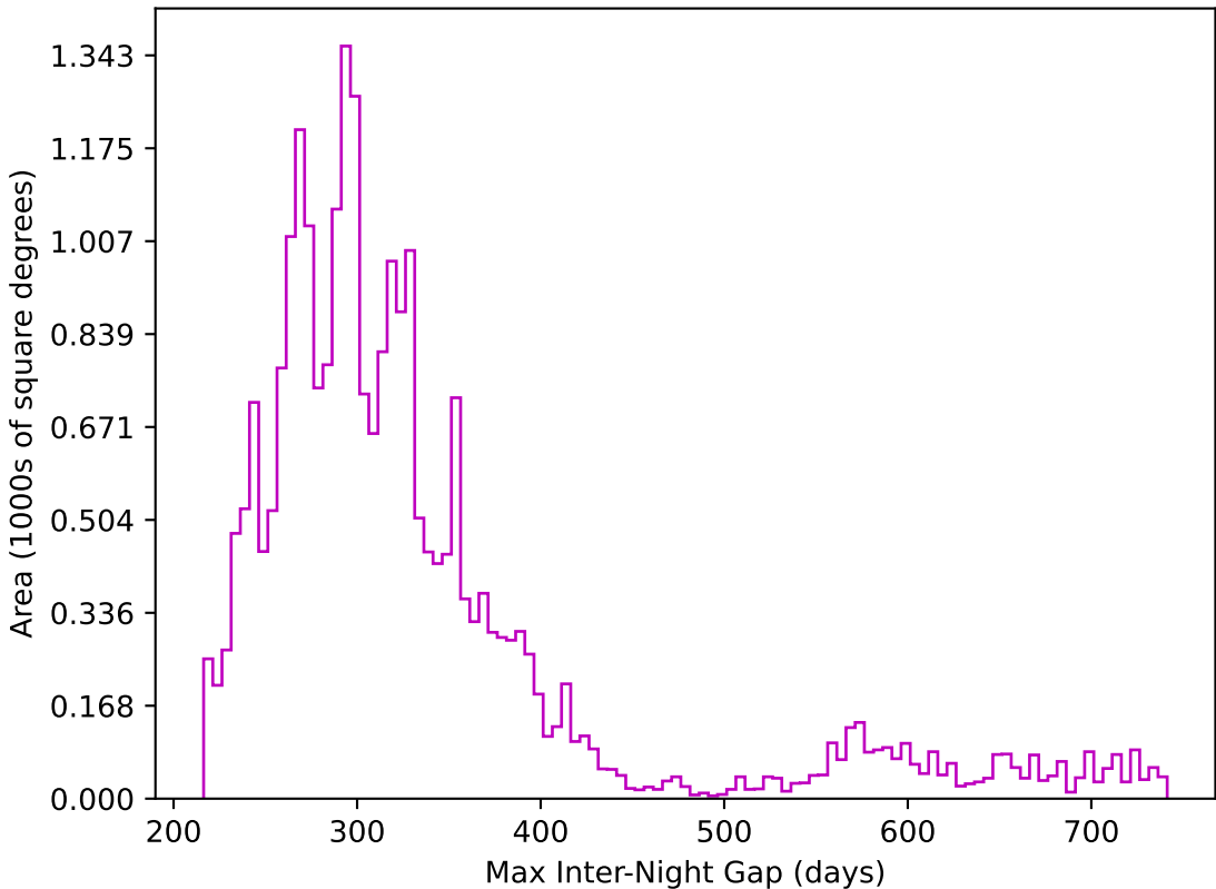
too_ignore_5_4v3.4_10yrs All sky z band: Max Inter-Night Gap
