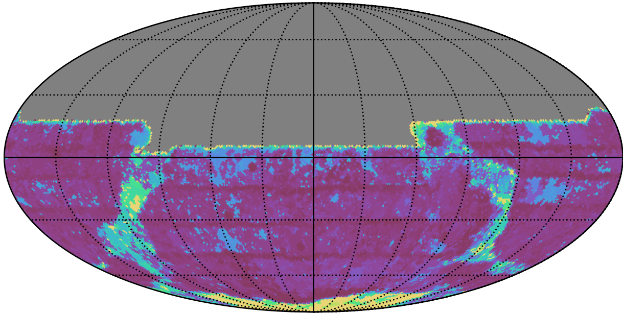
too_ignore_5_4v3.4_10yrs All sky y band: Max Inter-Night Gap
