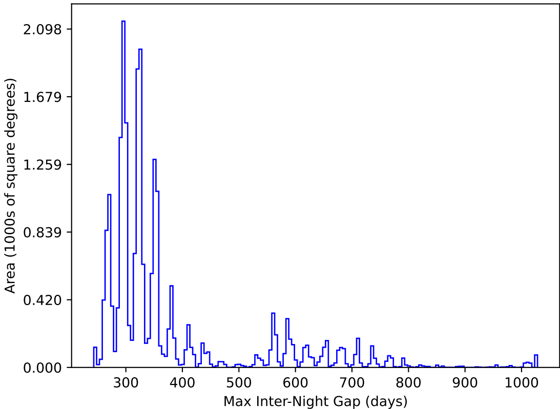
too_ignore_5_4v3.4_10yrs All sky y band: Max Inter-Night Gap
