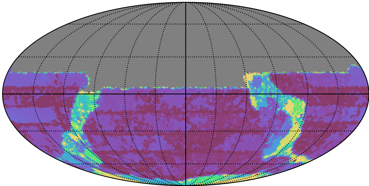
too_ignore_5_4v3.4_10yrs All sky u band: Max Inter-Night Gap
