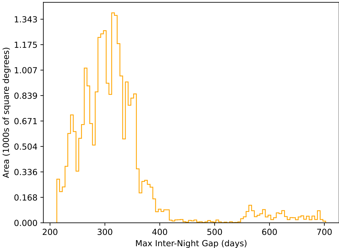
too_ignore_5_4v3.4_10yrs All sky r band: Max Inter-Night Gap
