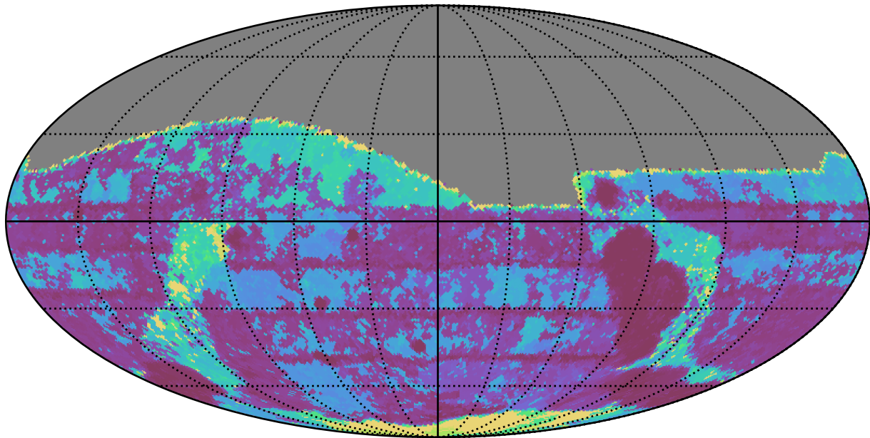
too_ignore_5_4v3.4_10yrs All sky g band: Max Inter-Night Gap
