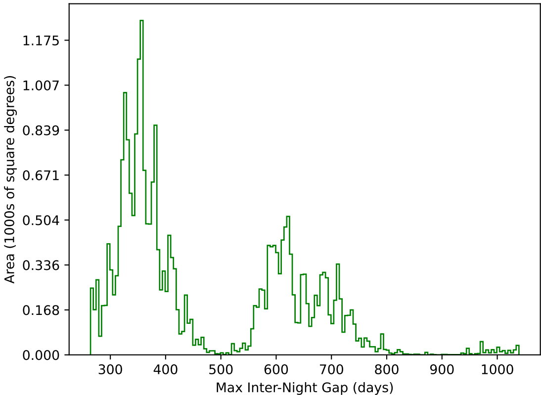
too_ignore_5_4v3.4_10yrs All sky g band: Max Inter-Night Gap
