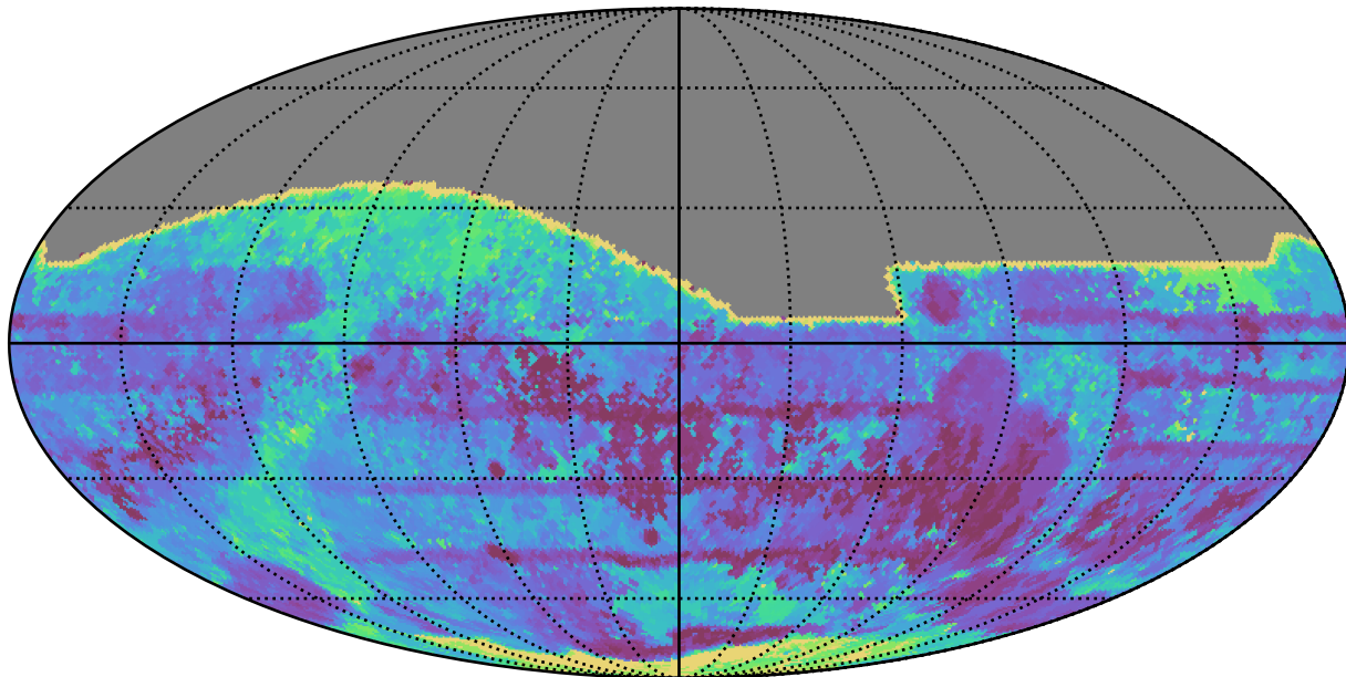
too_ignore_5_4v3.4_10yrs All sky all bands: Max Inter-Night Gap
