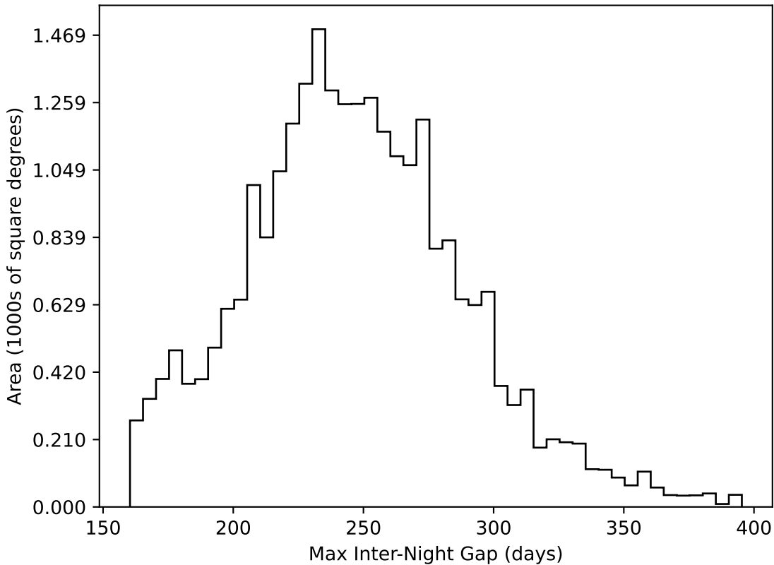
too_ignore_5_4v3.4_10yrs All sky all bands: Max Inter-Night Gap
