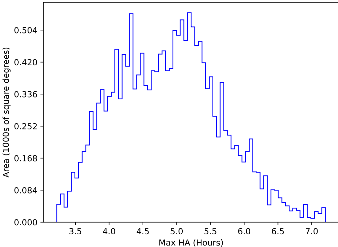
too_ignore_5_4v3.4_10yrs WFD z band: Max HA
