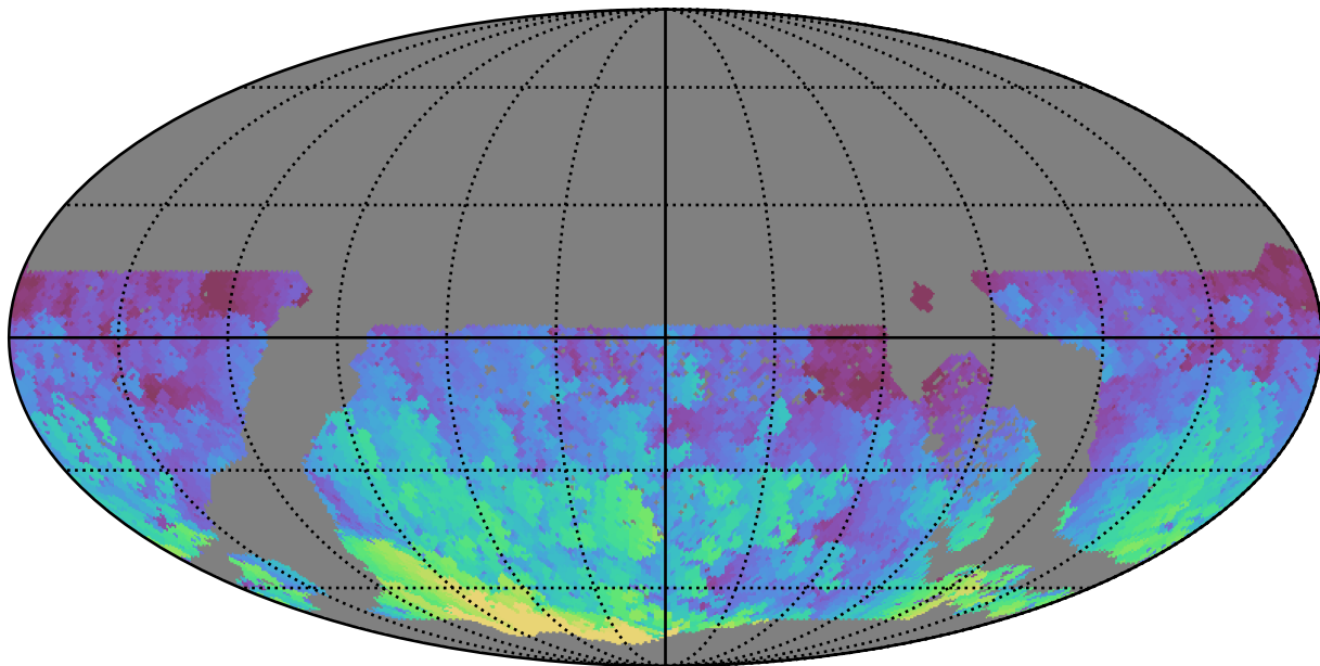
too_ignore_5_4v3.4_10yrs WFD u band: Max HA
