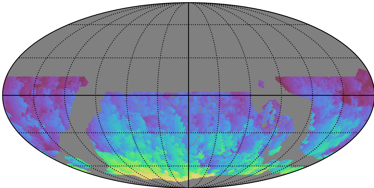
too_ignore_5_4v3.4_10yrs WFD r band: Max HA
