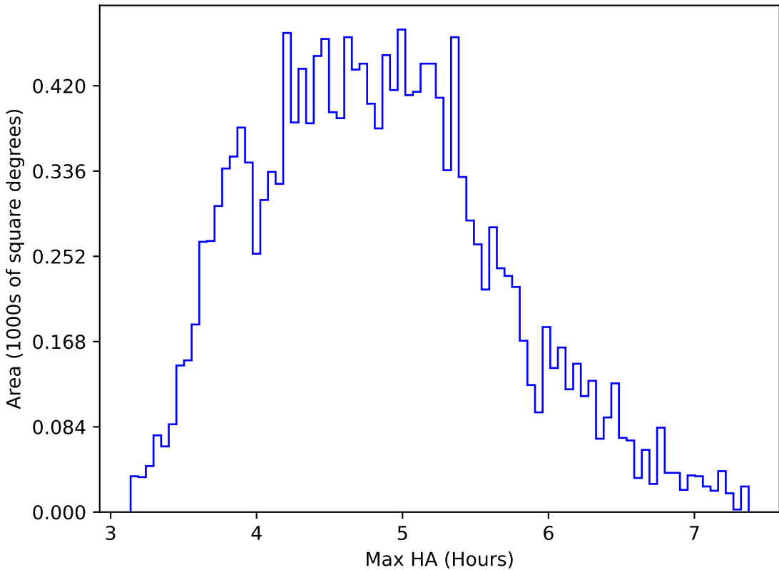
too_ignore_5_4v3.4_10yrs WFD i band: Max HA
