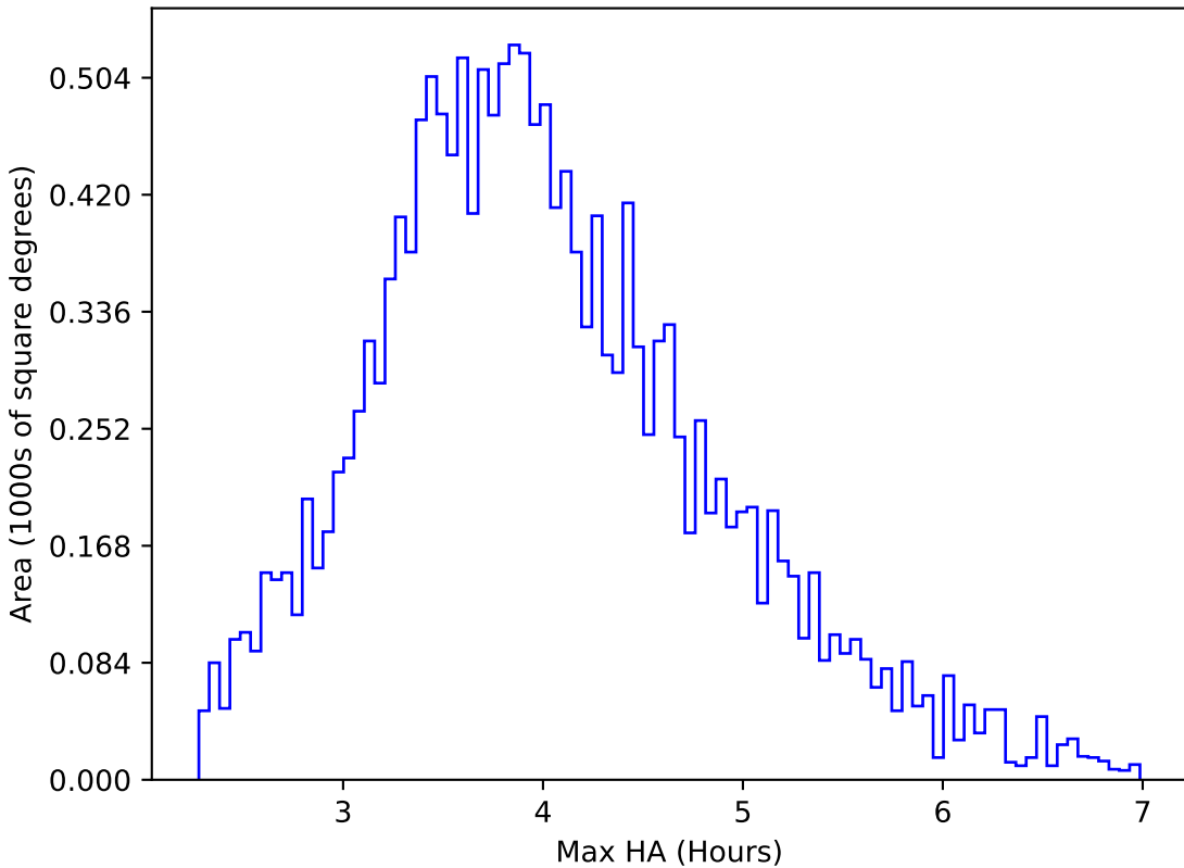
too_ignore_5_4v3.4_10yrs WFD g band: Max HA
