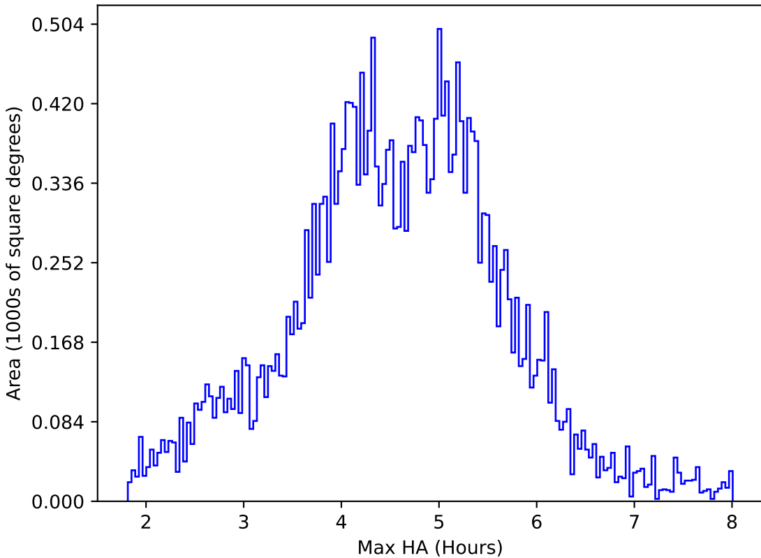
too_ignore_5_4v3.4_10yrs All sky z band: Max HA
