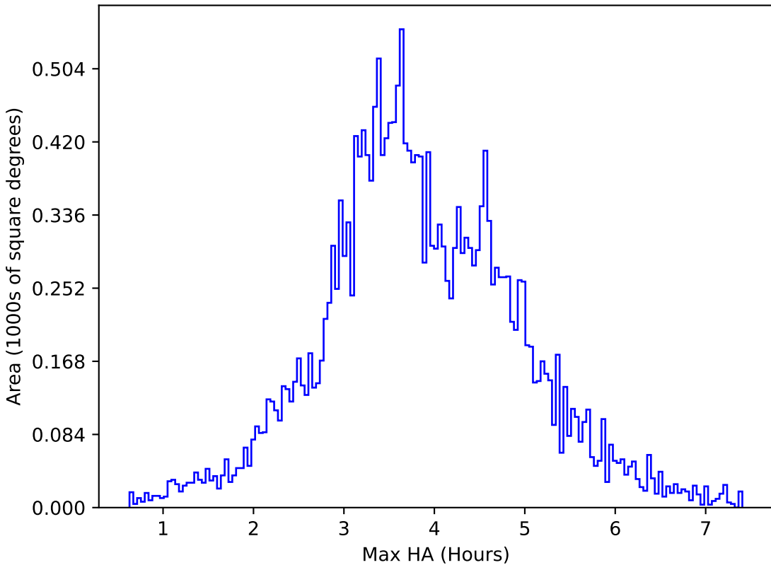
too_ignore_5_4v3.4_10yrs All sky u band: Max HA
