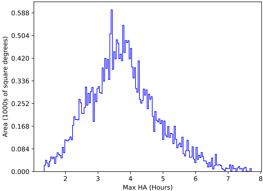
too_ignore_5_4v3.4_10yrs All sky g band: Max HA
