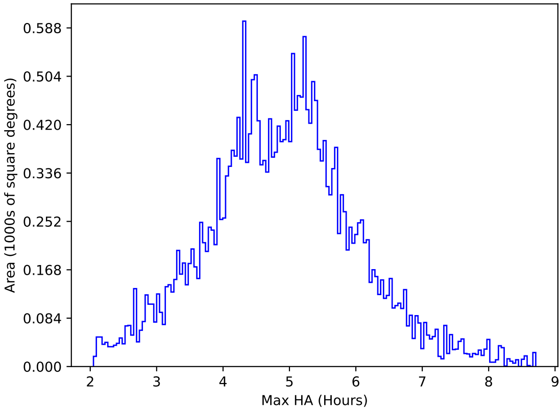
too_ignore_5_4v3.4_10yrs All sky all bands: Max HA
