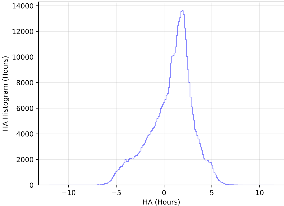
too_ignore_5_4v3.4_10yrs WFD z band: HA Histogram
