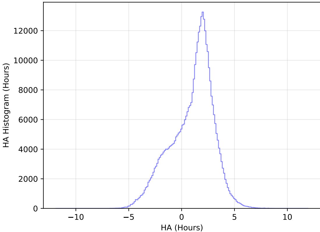
too_ignore_5_4v3.4_10yrs WFD y band: HA Histogram
