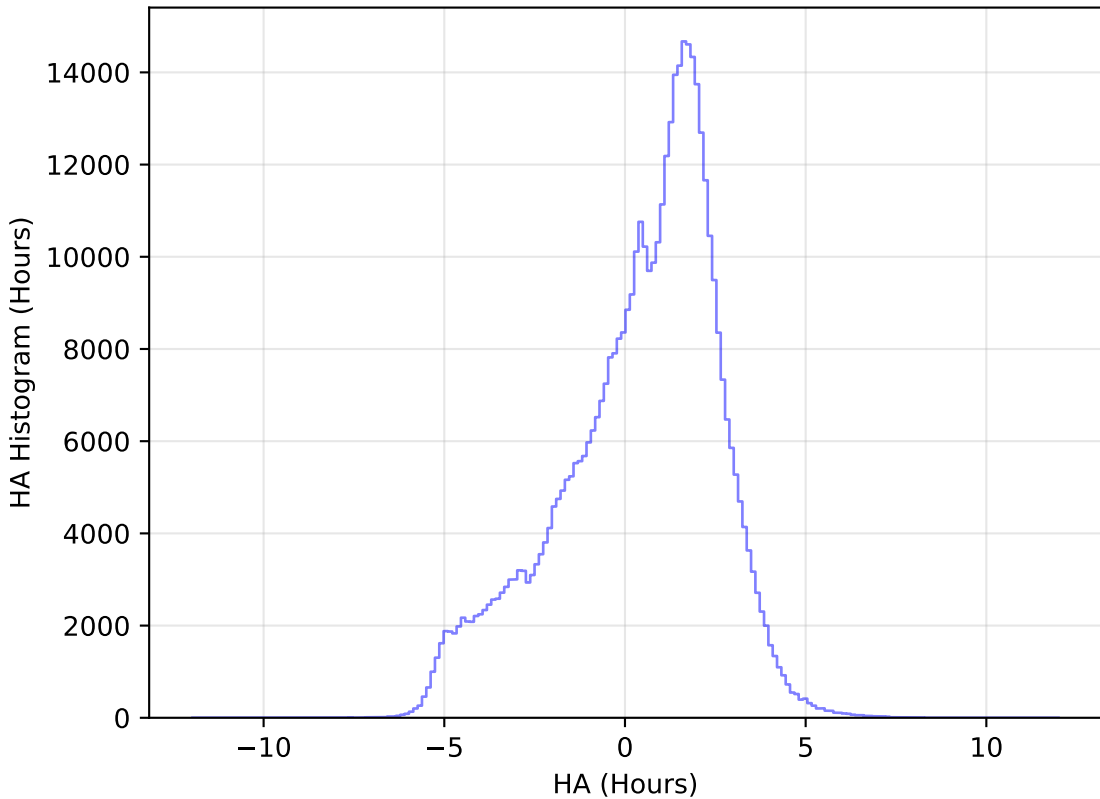
too_ignore_5_4v3.4_10yrs WFD r band: HA Histogram
