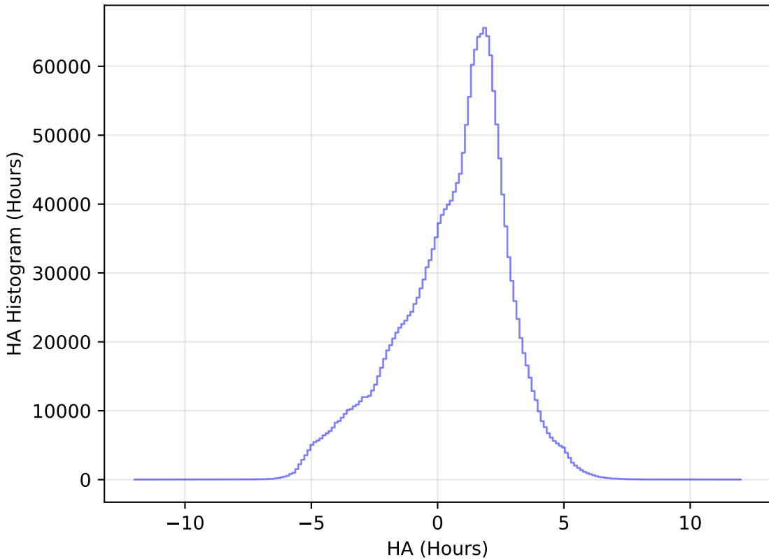
too_ignore_5_4v3.4_10yrs WFD all bands: HA Histogram
