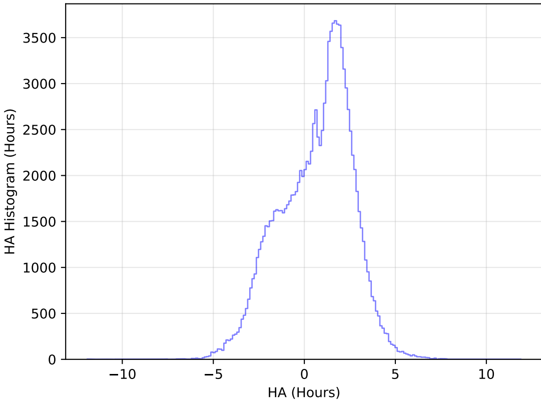
too_ignore_5_4v3.4_10yrs All sky u band: HA Histogram
