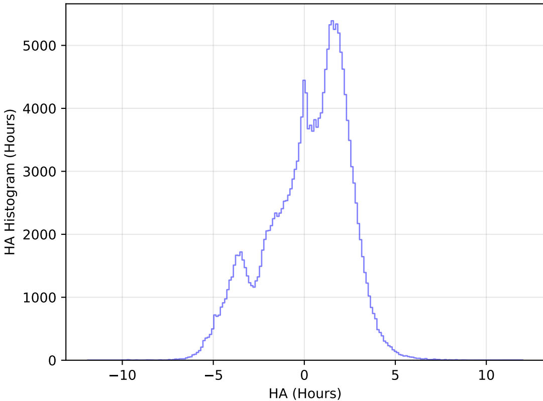
too_ignore_5_4v3.4_10yrs All sky g band: HA Histogram
