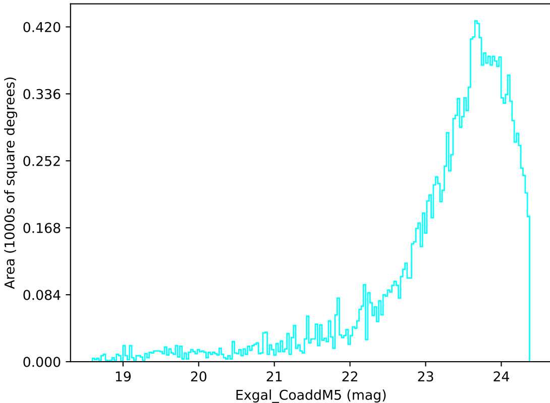
too_ignore_5_4v3.4_10yrs Yr 3-4 u band: Exgal_CoaddM5
