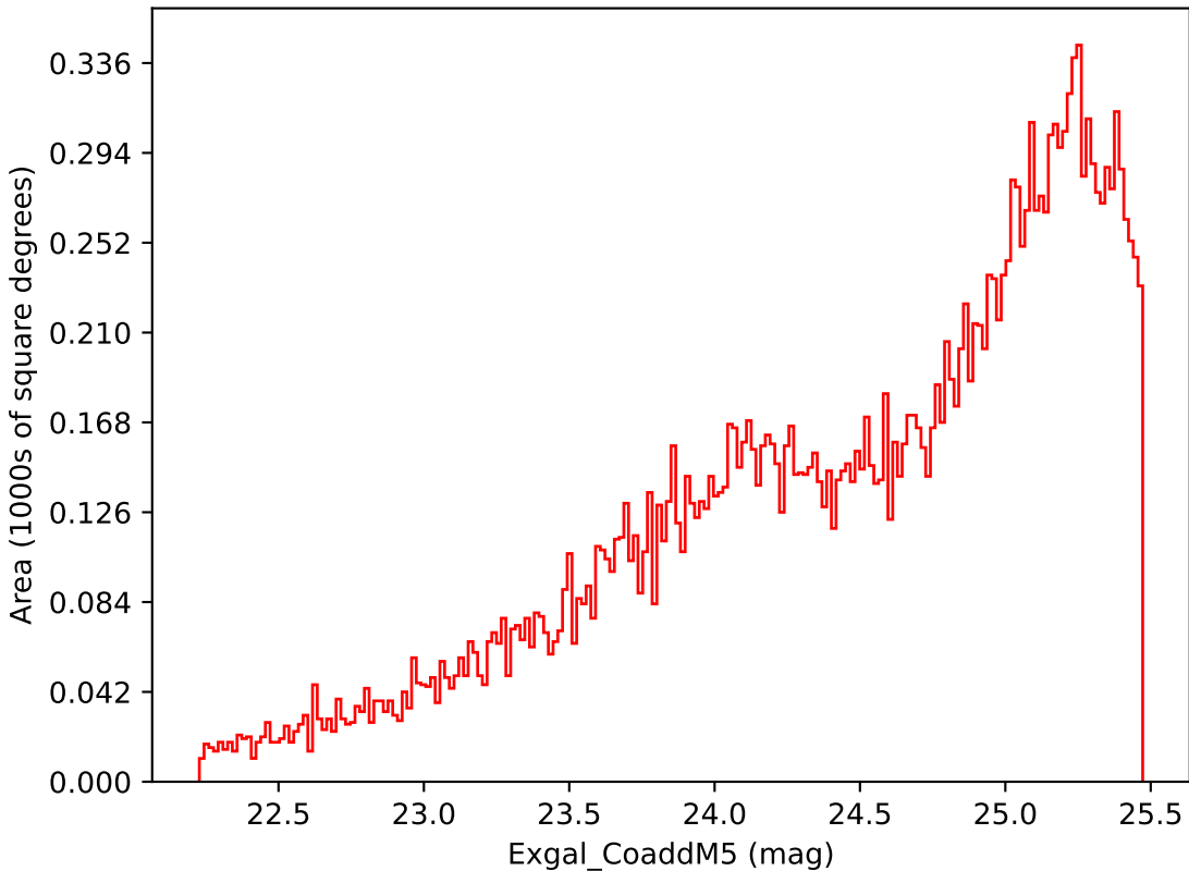
too_ignore_5_4v3.4_10yrs Yr 3-4 i band: Exgal_CoaddM5
