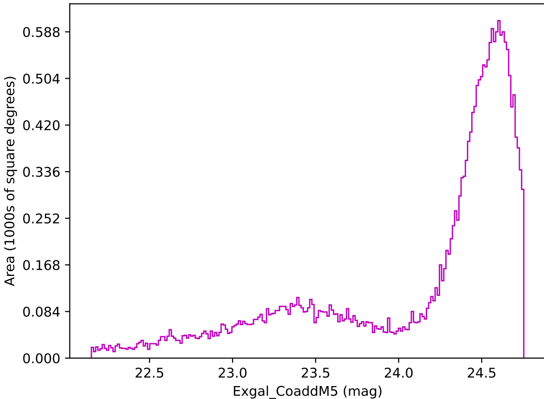
too_ignore_5_4v3.4_10yrs Yr 1 z band: Exgal_CoaddM5
