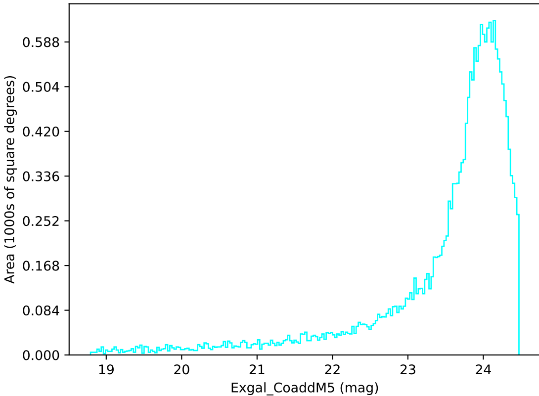
too_ignore_5_4v3.4_10yrs Yr 1 u band: Exgal_CoaddM5
