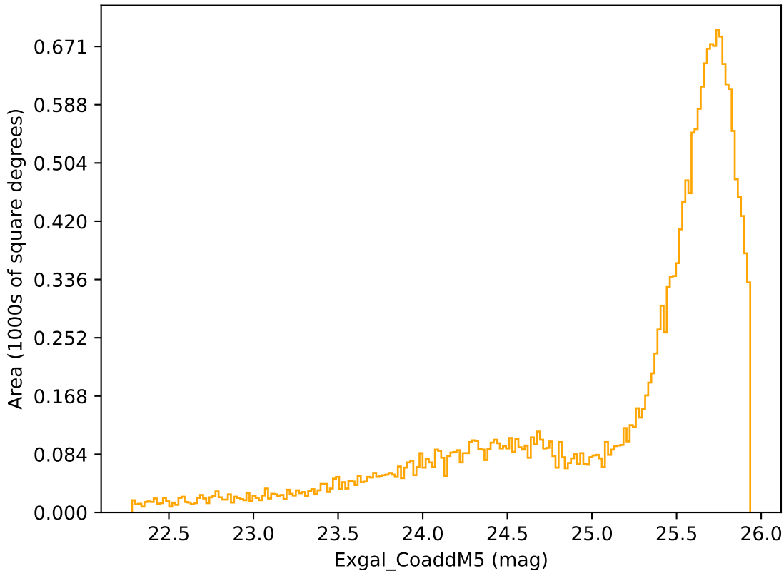
too_ignore_5_4v3.4_10yrs Yr 1 r band: Exgal_CoaddM5
