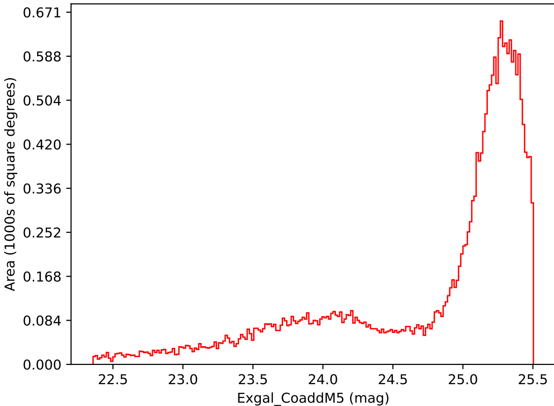
too_ignore_5_4v3.4_10yrs Yr 1 i band: Exgal_CoaddM5
