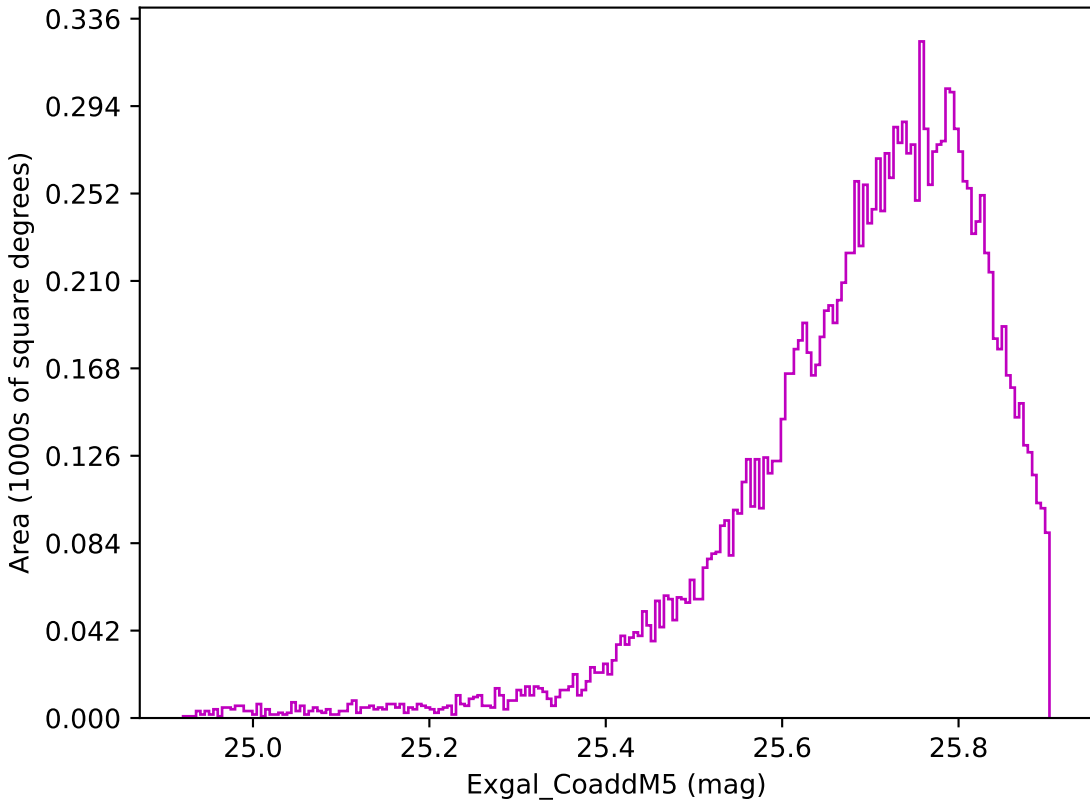
too_ignore_5_4v3.4_10yrs WFD z band: Exgal_CoaddM5
