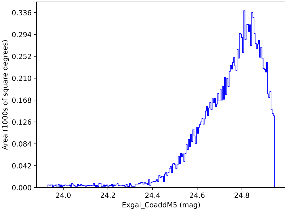
too_ignore_5_4v3.4_10yrs WFD y band: Exgal_CoaddM5
