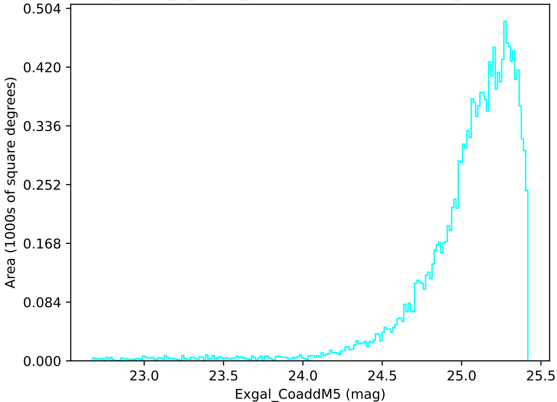
too_ignore_5_4v3.4_10yrs WFD u band: Exgal_CoaddM5
