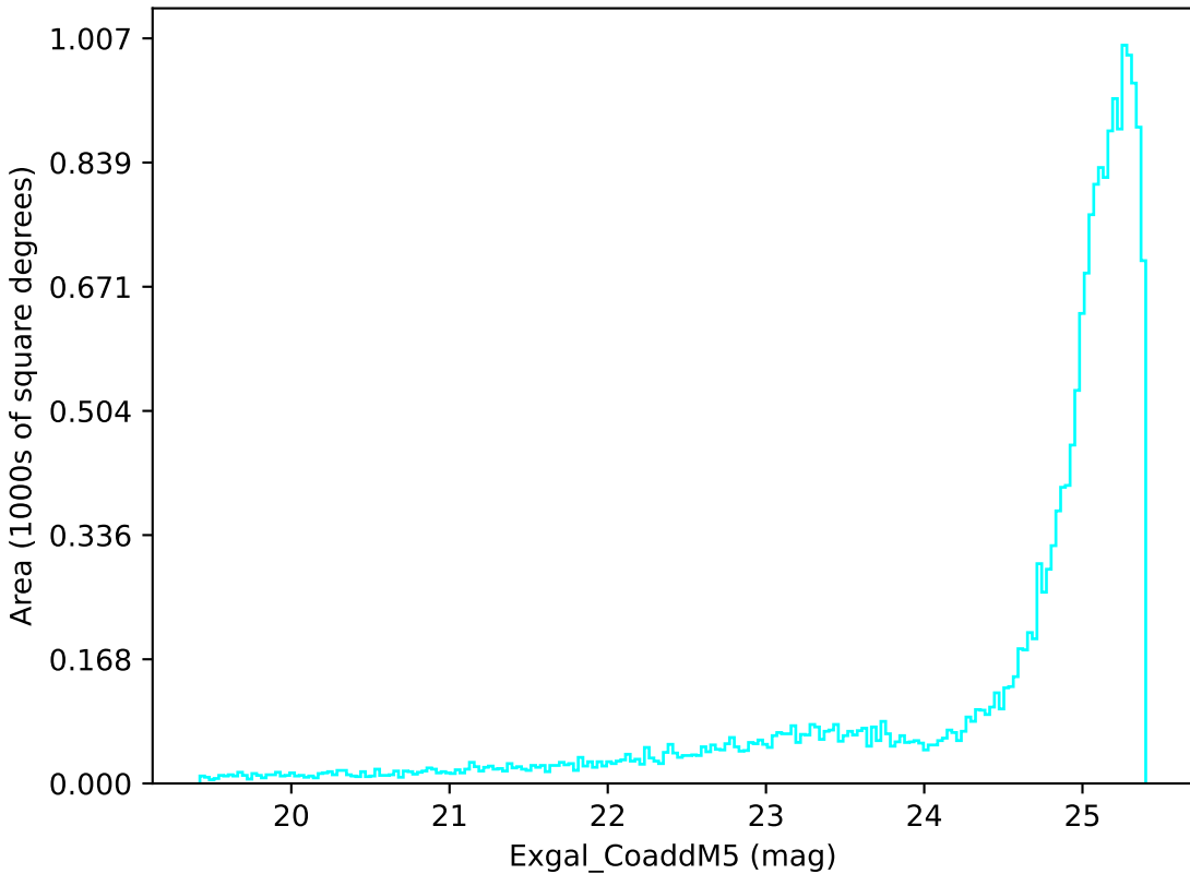
too_ignore_5_4v3.4_10yrs All sky u band: Exgal_CoaddM5
