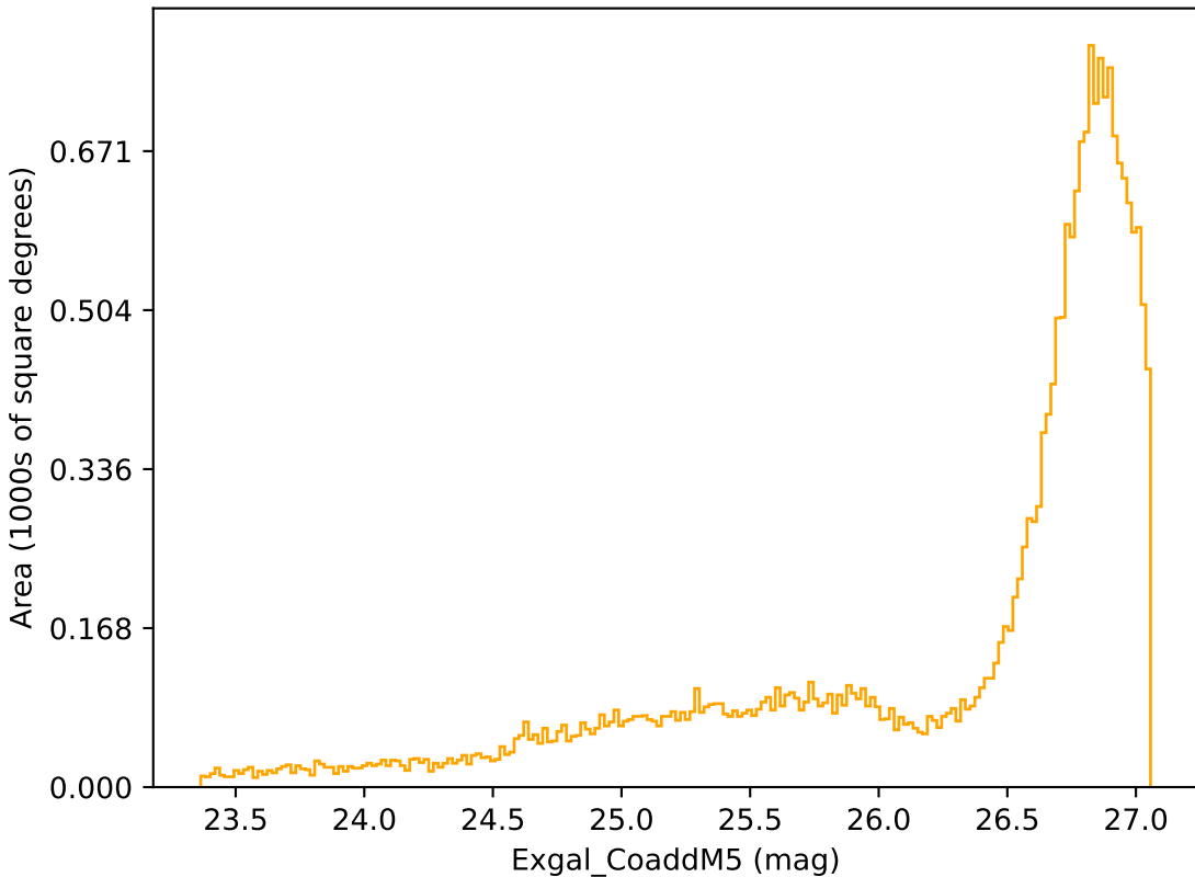
too_ignore_5_4v3.4_10yrs All sky r band: Exgal_CoaddM5
