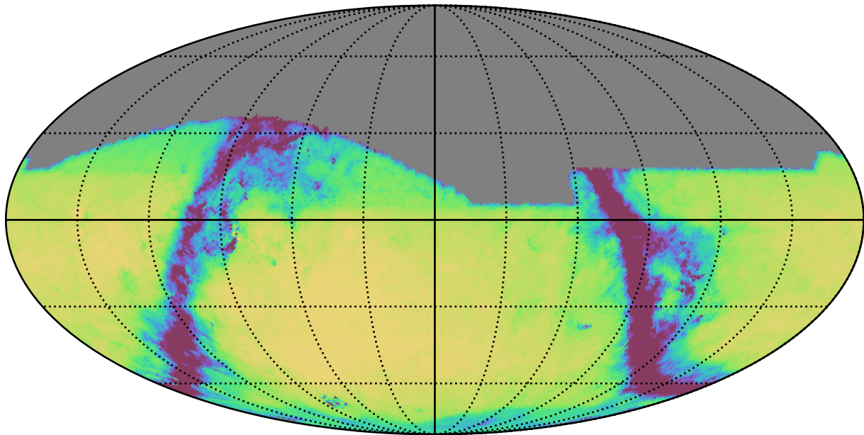
too_ignore_5_4v3.4_10yrs All sky g band: Exgal_CoaddM5
