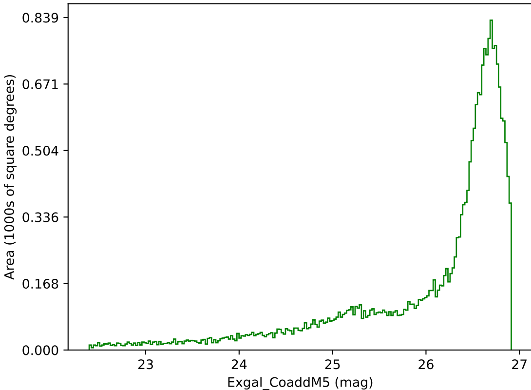
too_ignore_5_4v3.4_10yrs All sky g band: Exgal_CoaddM5
