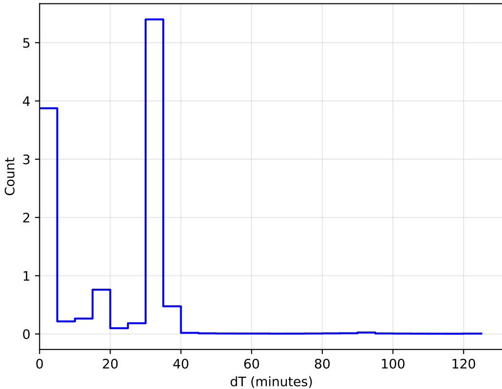
1e6 too_ignore_5_4v3.4_10yrs WFD: DeltaT Histogram
