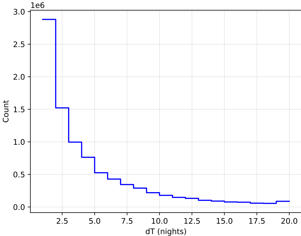
too_ignore_5_4v3.4_10yrs All sky all bands: DeltaNight Histogram
