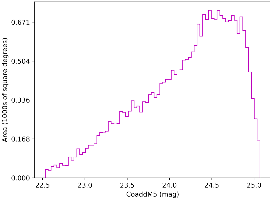
too_ignore_5_4v3.4_10yrs Yr 3-4 z band: CoaddM5
