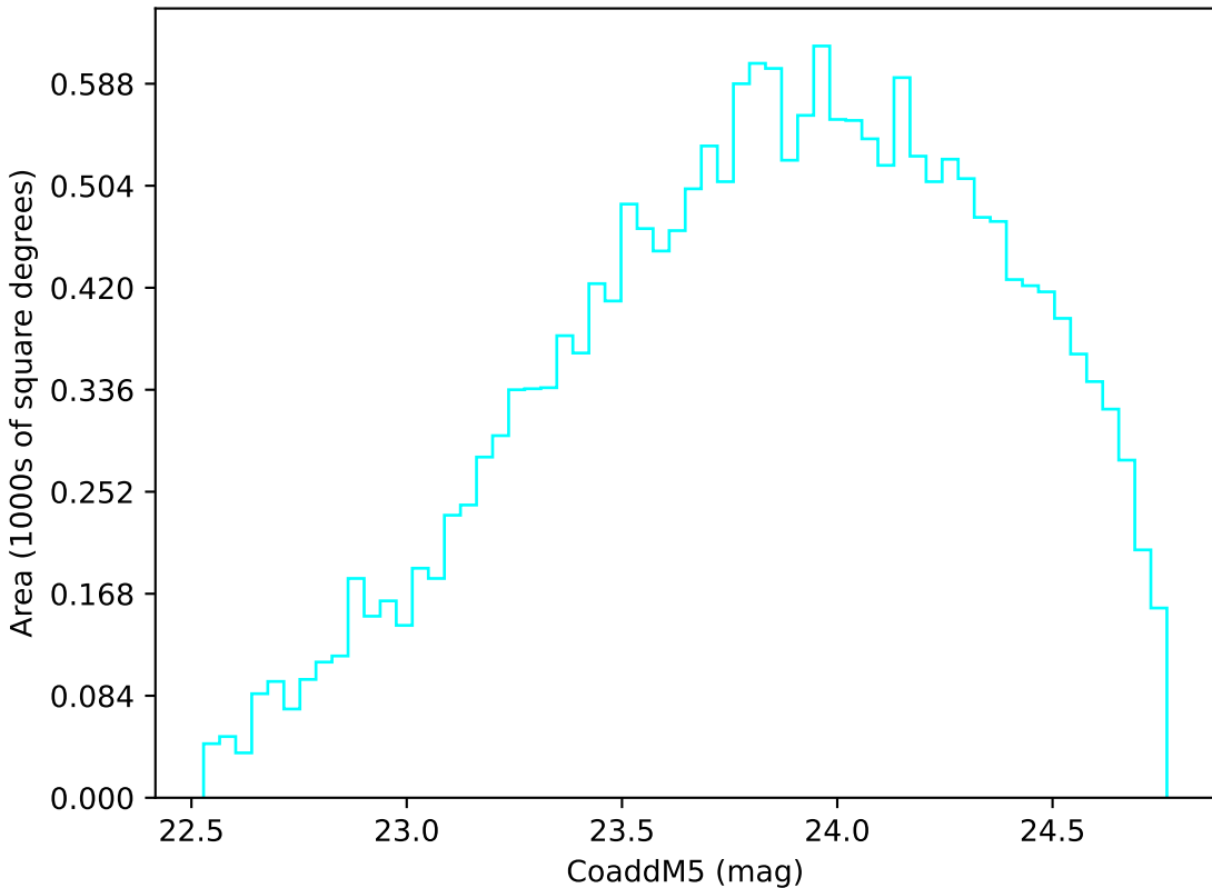
too_ignore_5_4v3.4_10yrs Yr 3-4 u band: CoaddM5
