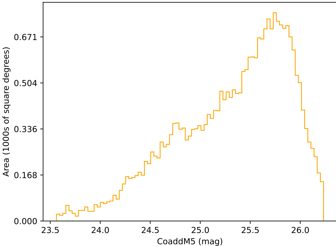
too_ignore_5_4v3.4_10yrs Yr 3-4 r band: CoaddM5
