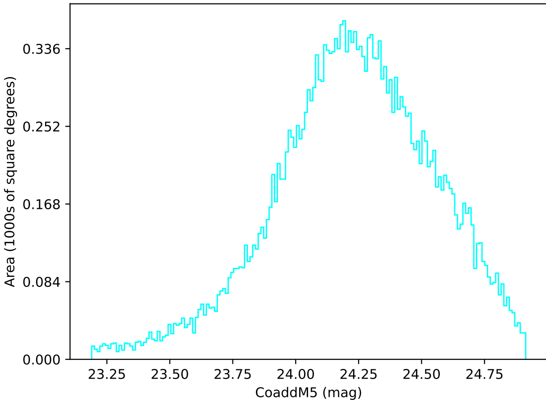
too_ignore_5_4v3.4_10yrs Yr 1 u band: CoaddM5
