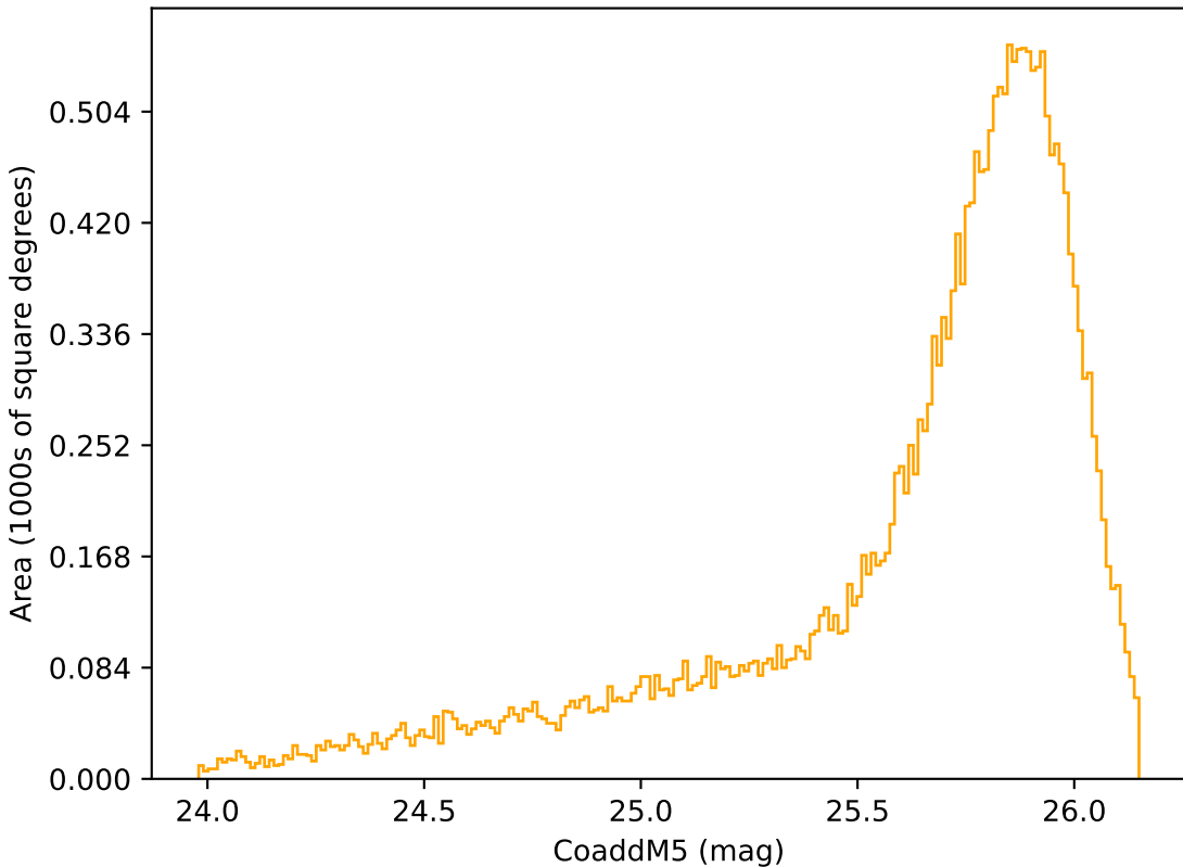
too_ignore_5_4v3.4_10yrs Yr 1 r band: CoaddM5
