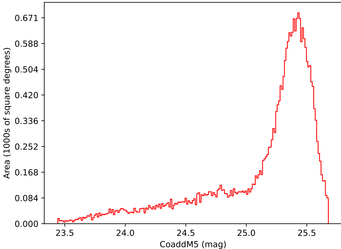
too_ignore_5_4v3.4_10yrs Yr 1 i band: CoaddM5
