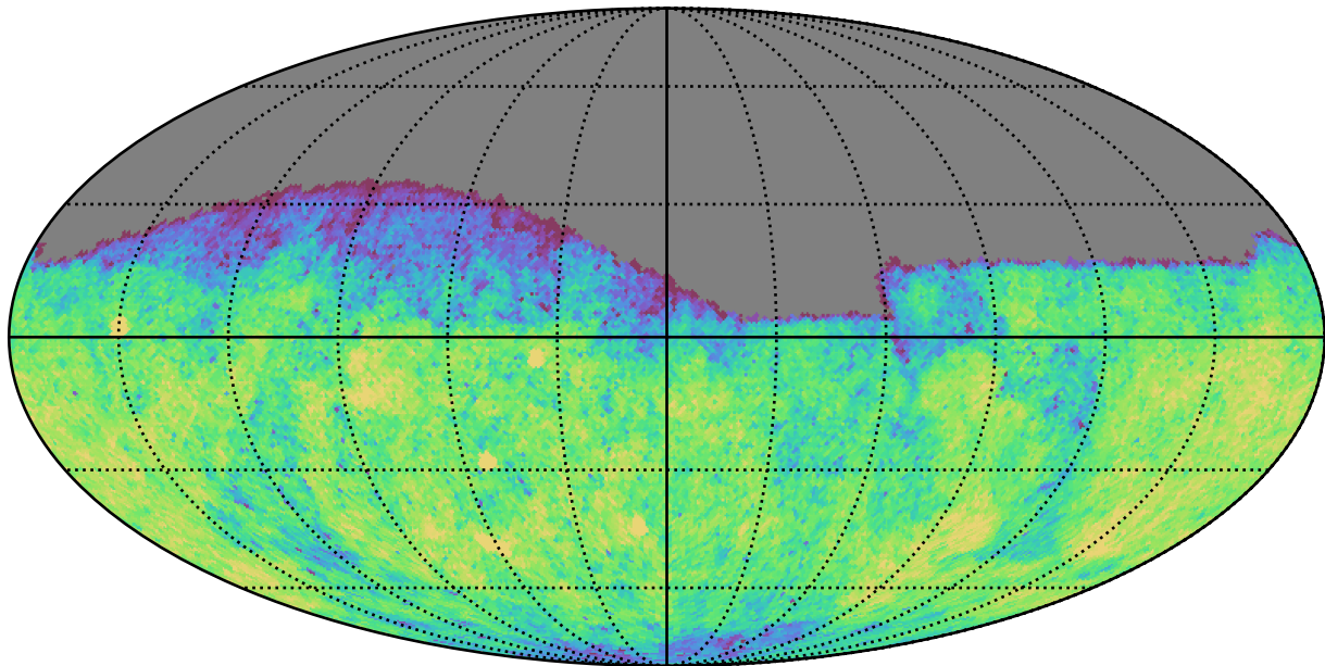
too_ignore_5_4v3.4_10yrs Yr 1 g band: CoaddM5
