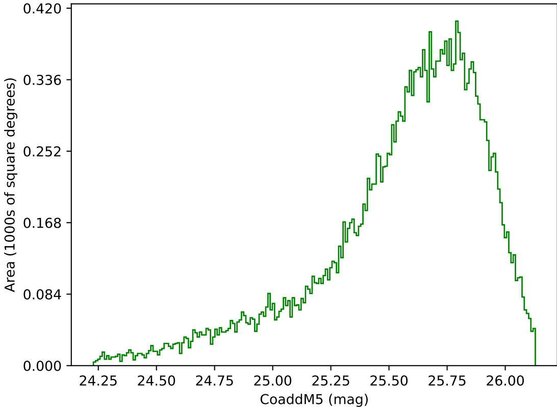
too_ignore_5_4v3.4_10yrs Yr 1 g band: CoaddM5
