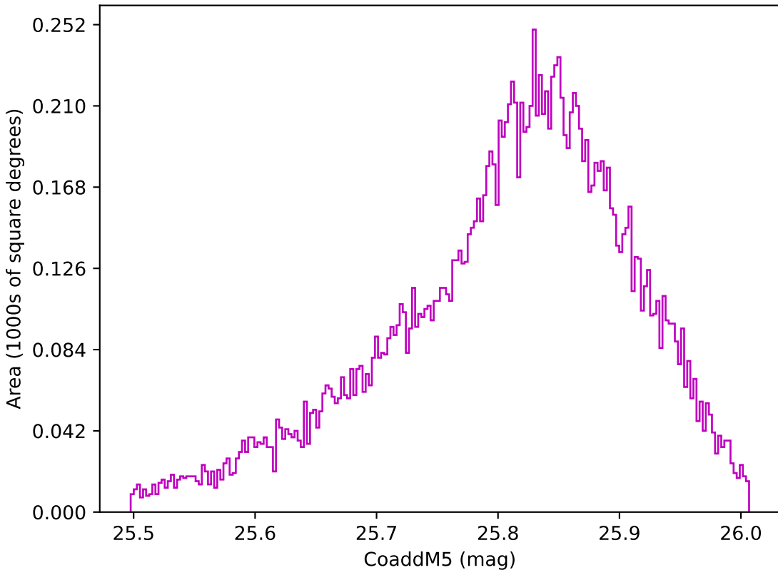
too_ignore_5_4v3.4_10yrs WFD z band: CoaddM5
