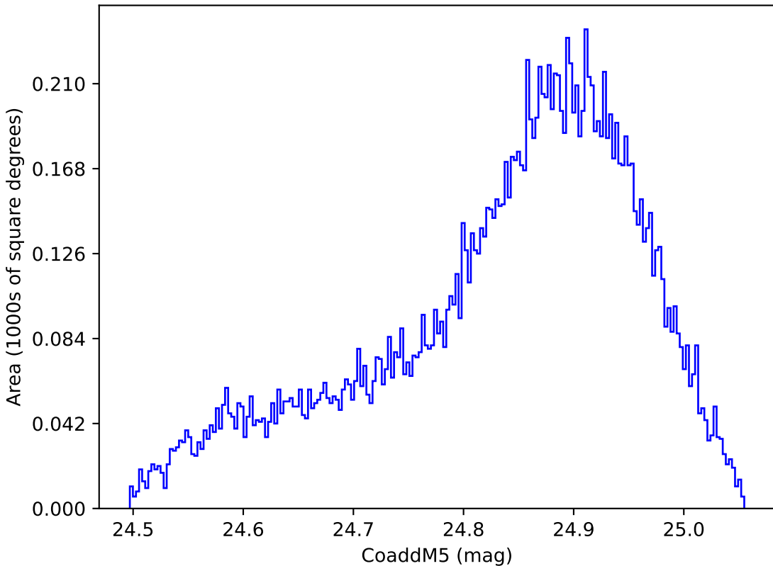
too_ignore_5_4v3.4_10yrs WFD y band: CoaddM5
