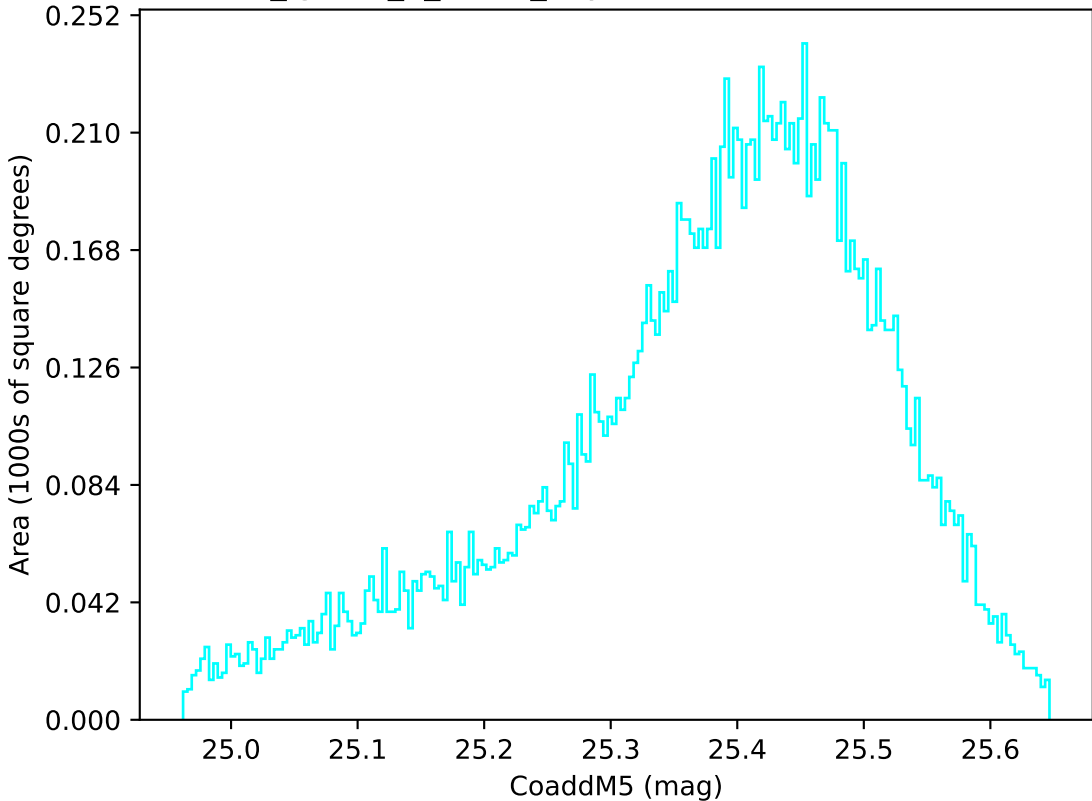
too_ignore_5_4v3.4_10yrs WFD u band: CoaddM5
